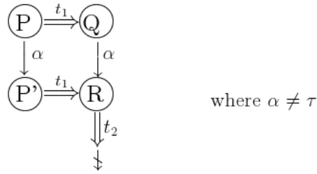
Figure 3.3: Confluence from P to R
