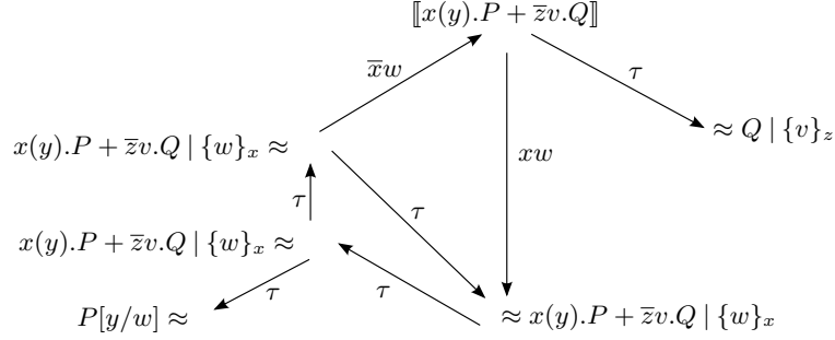
Fig. 2. Transitions of the \pi_a encoding of the \pi_{\mathfrak{B}} sum in Figure 1.
