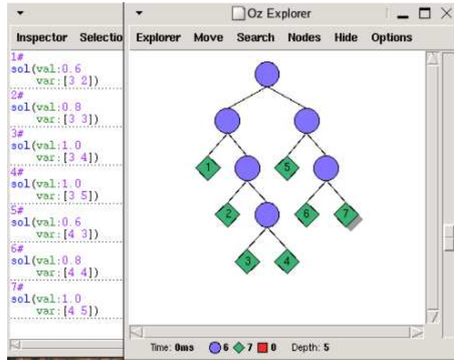
Figure 1. Exploration tree
